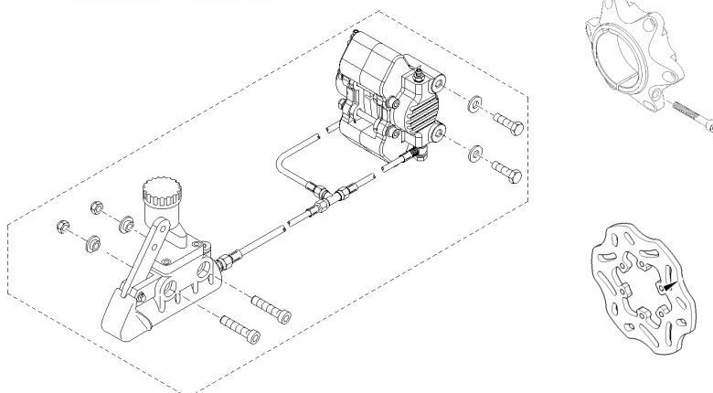
IMPIANTO FRENO EASYKART 100/125 R-I 38 H8/P22-SR/LS 510
